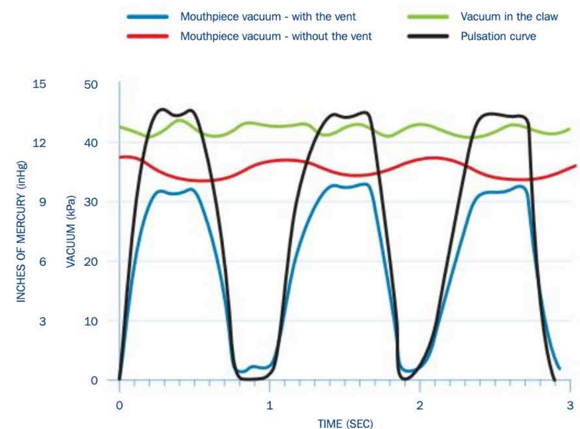
PULSATION AND VACUUM CURVES THROUGH THE MILKING CYCLE - AT LOW FLOW
