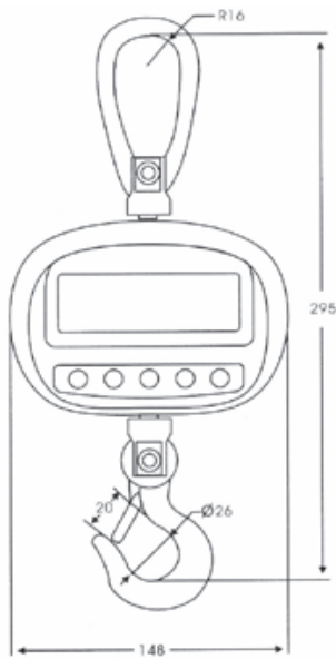
Figure 1 (unit: mm)
