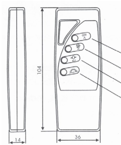
Figure 2 (unit: mm)
